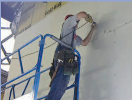
Drywall attaches easily to the embedded galvanized (G-60) furring strips (25ga).
